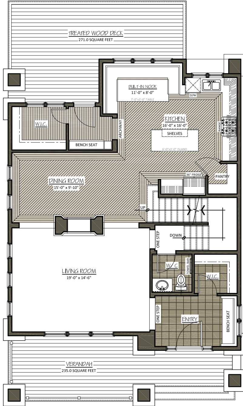
COOPERS TOWN SPEC #2 PROPOSED MAIN FLOOR 1,150.7 SQUARE FEET 1/8" = 1'-0" SCALE
